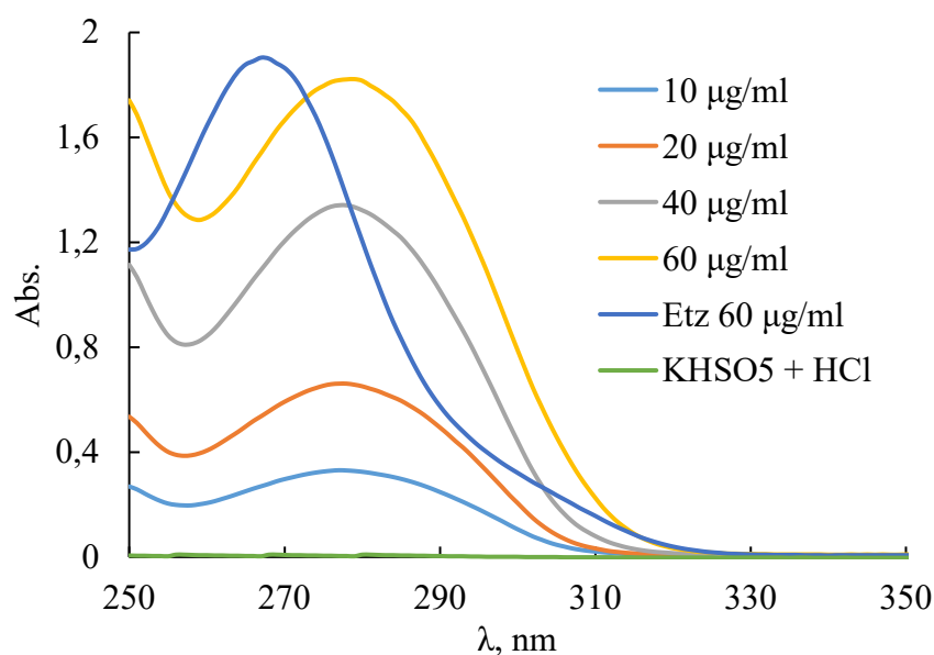
Fig. 3 The spectra of Ethacizine (60 \mu\text{g/mL} ), Ethacizine after transformation to the corresponding sulfoxide (10-60 \mu\text{g/mL} ) and the reagent ( c(\text{KHSO}_5) = 4,8 \cdot 10^{-4} \text{ mol/L} ). Solvent water, pH=2,1.
