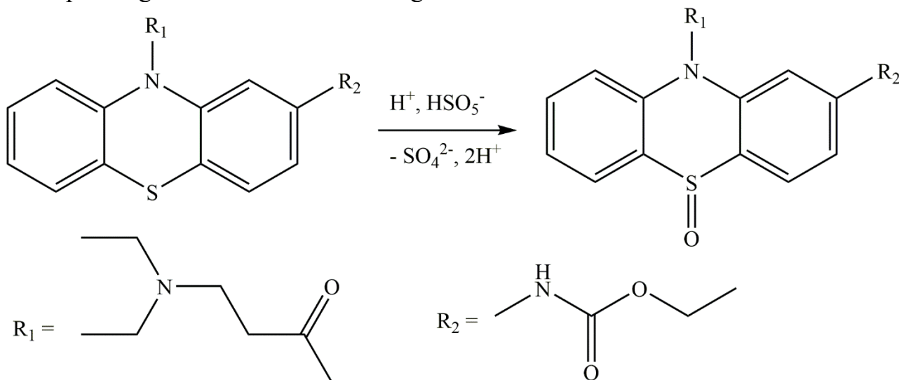
Fig. 2 The scheme of the oxidation process of Ethacizine to the corresponding sulfoxide using Oxone
