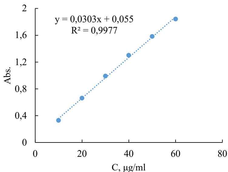
Fig. 4 Calibration curve for determination of Ethacizine HCl as its sulfoxide at \lambda_{\max} = 279\text{ nm} , l = 1\text{ cm} , c(\text{KHSO}_5) = 4.8 \times 10^{-4}\text{ M} , \text{pH} = 2.1
